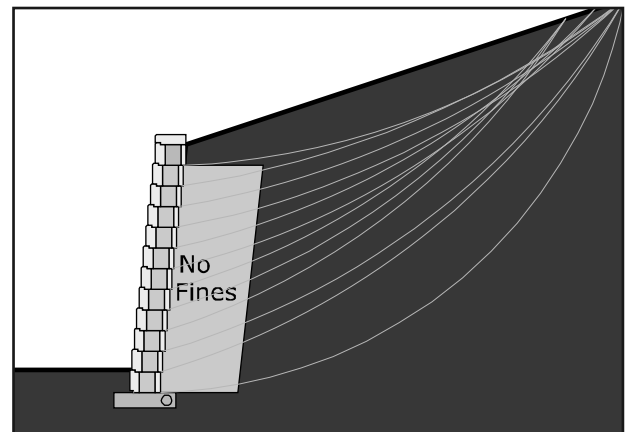
Figure D-6. NFC - ICS Analysis
