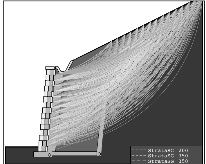
Figure 7-13. ICS Pressure Map Diagram
