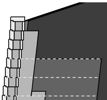
Standard gravity wall above geogrid wall
